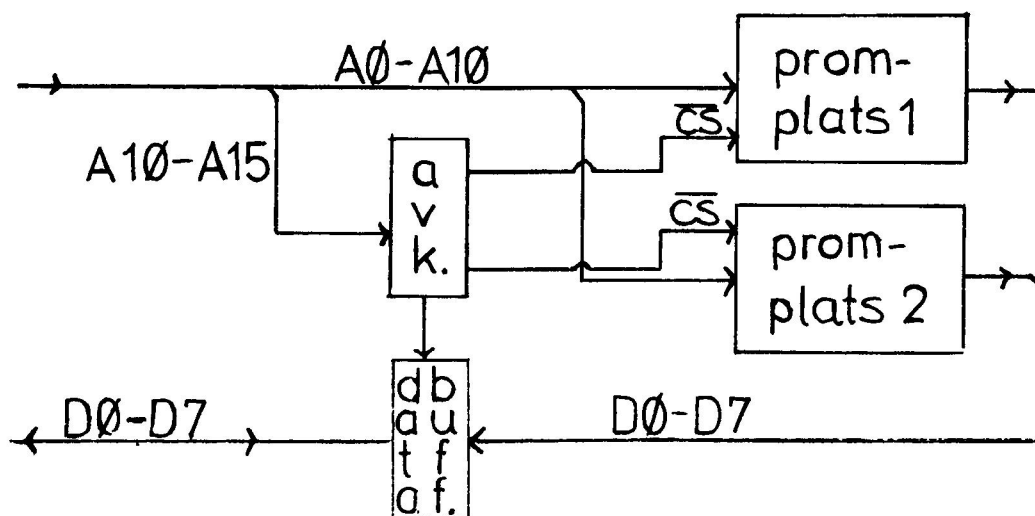
Blockschema minnesexpansion
