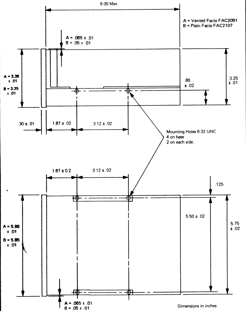
FIGURE 7 Mounting details
