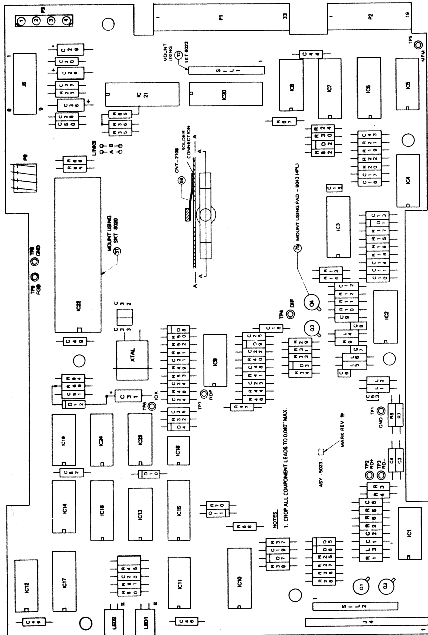
FIGURE 23 Master PCB layout
