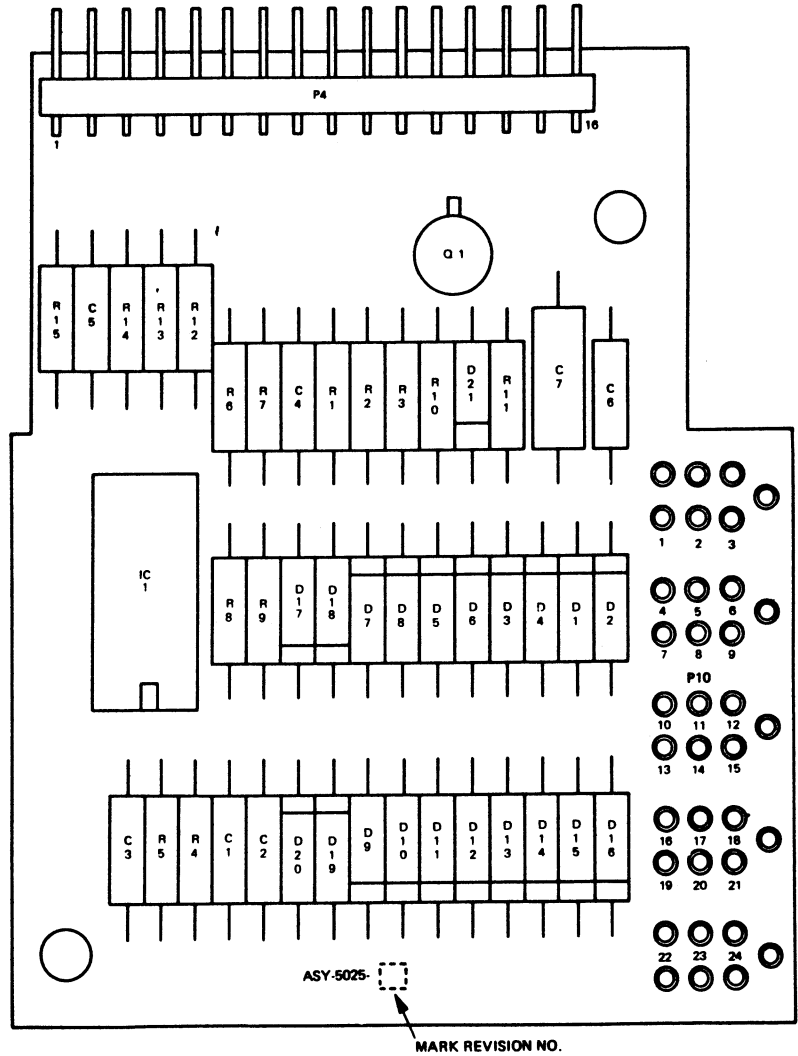
FIGURE 24 Pre-amplifier PCB layout
