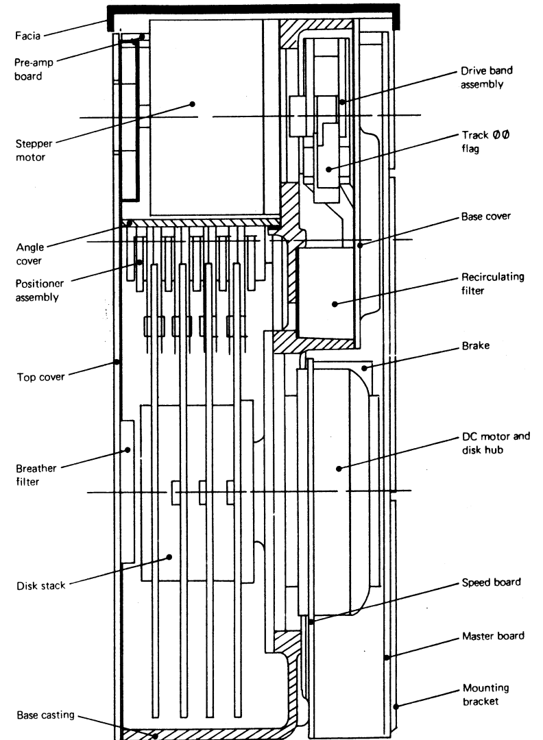
FIGURE 10 Non-planar section of RO 204
