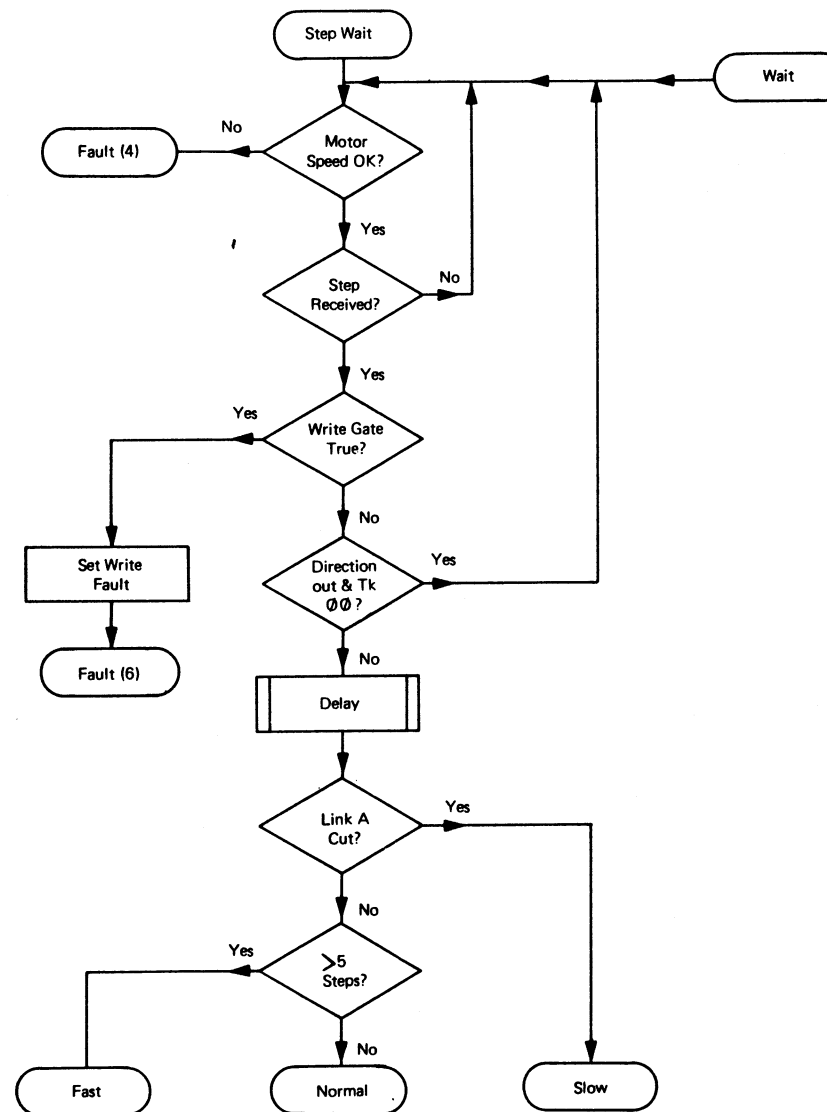
FIGURE 22(a) Step flow chart
