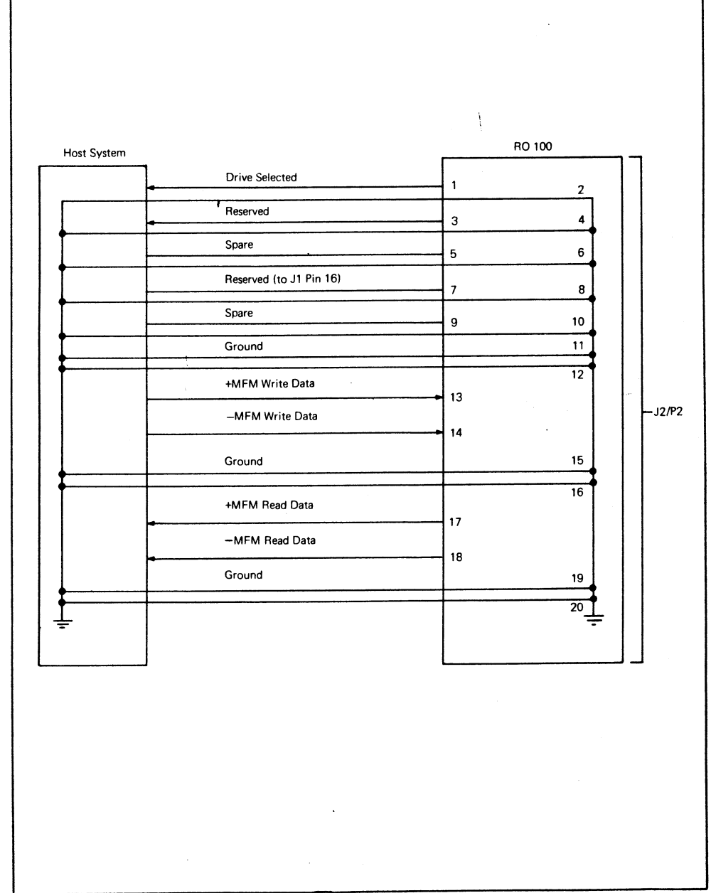
FIGURE 6 Data bus
