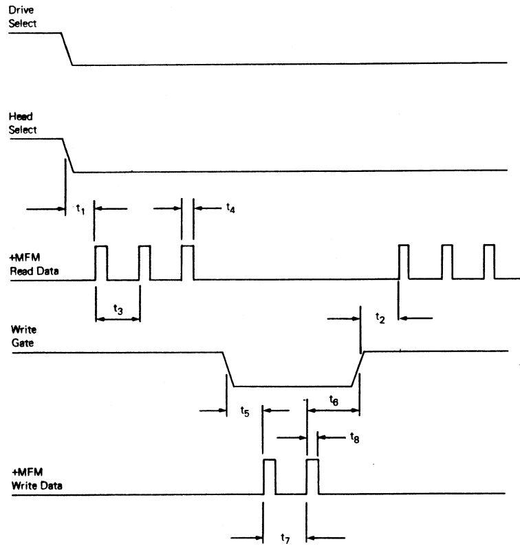
FIGURE 15 Read/Write data timing
