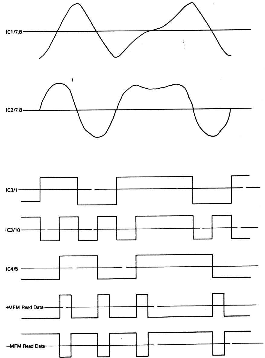
FIGURE 14 Read channel signals
