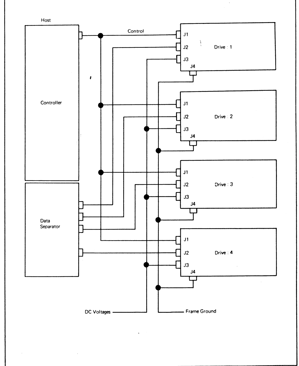
FIGURE 8 System with 4 drives
