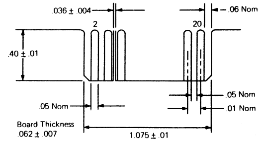
FIGURE 3 J2 Connector – Data
