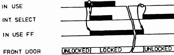
FIG. 2 - 13 TIMING DIAGRAM DOOR LOCK LATCH OPTION
