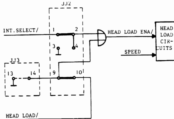
FIG. 2 - 10 SELECTED HEAD LOAD OPTION
