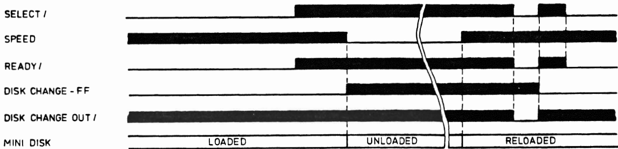
FIGURE 2 - 15 TIMING DIAGRAM DISK CHANGE LOGIC
