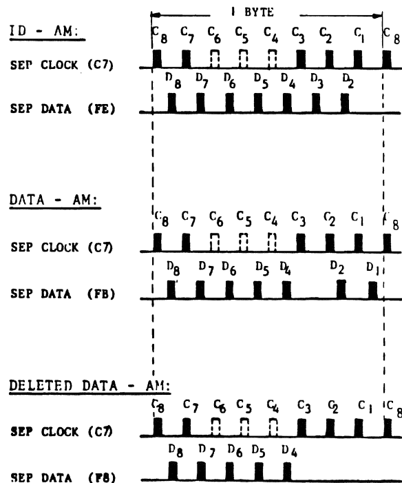
FIG. 1 - 5 ADDRESS MARK PATTERNS
